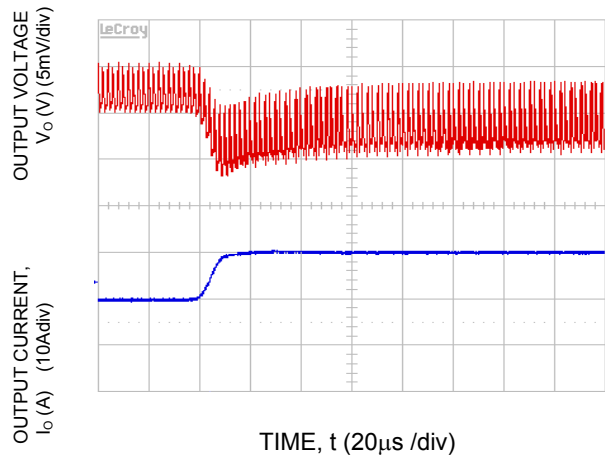
Fig-48. Transient Response to Dynamic Load Change from 50% to 100% at 12Vin, C_{out}= 1 \times 47\mu F + 11 \times 330\mu F , C_{Tune}=47nF , R_{Tune}=178\Omega
