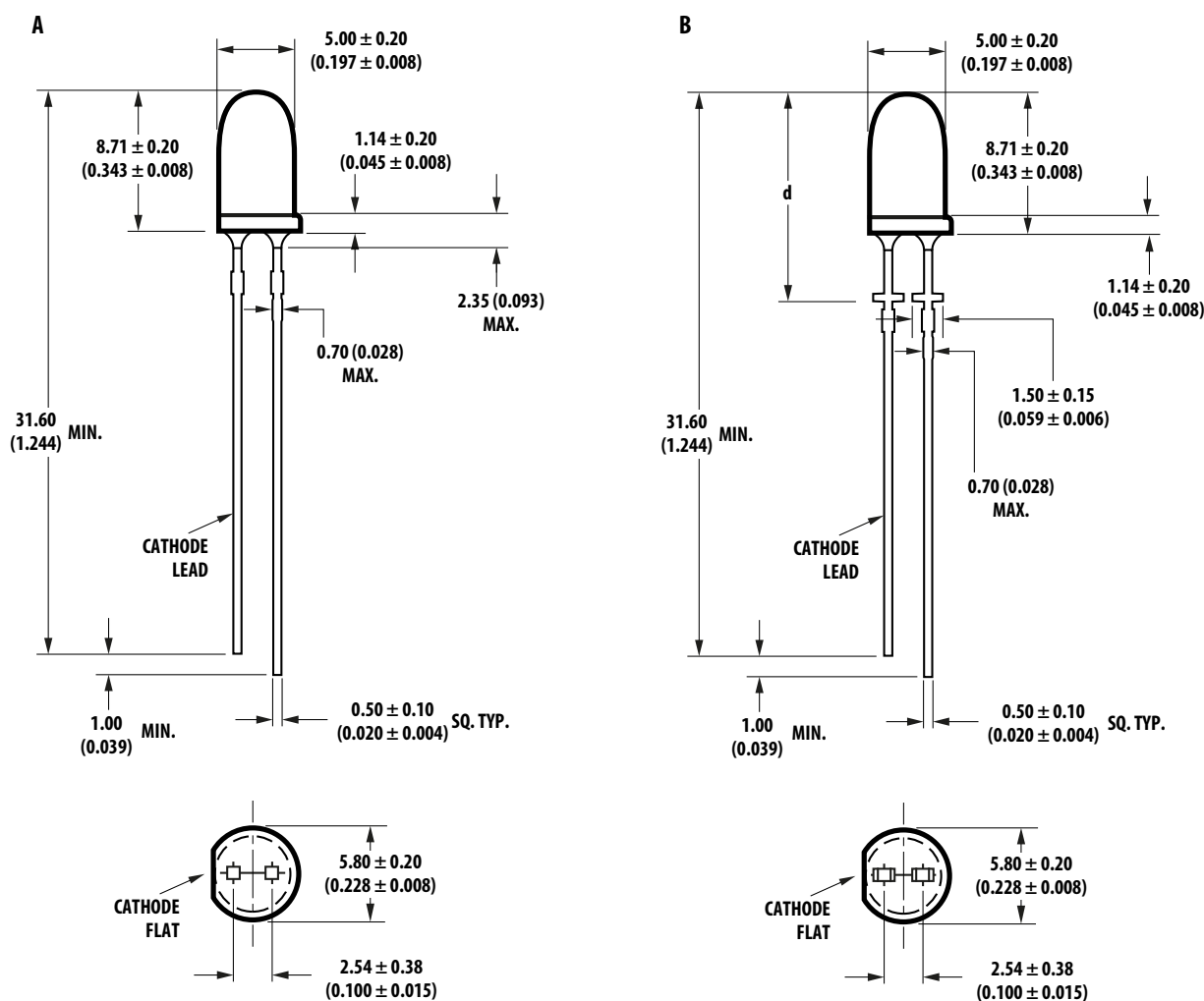
Figure 1: Package Dimensions
