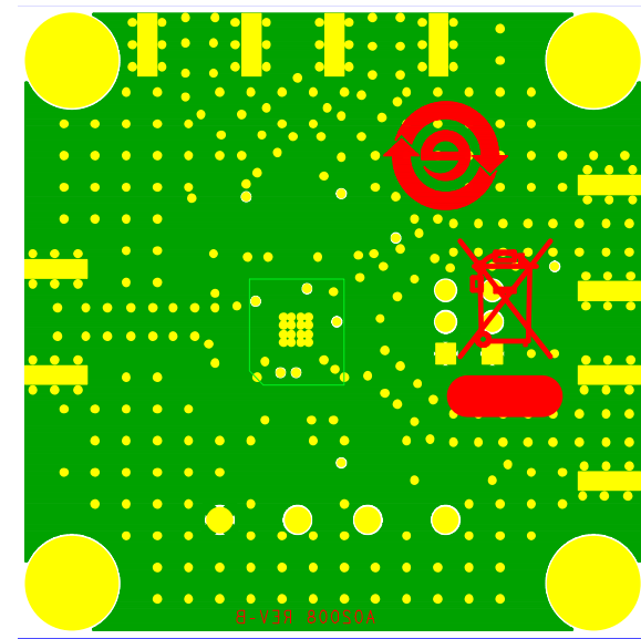
Figure 56. Evaluation Board Bottom Layer
