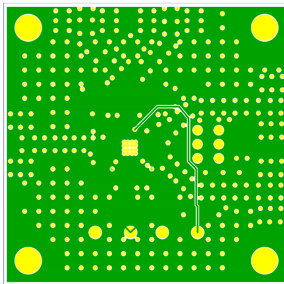
Figure 55. Evaluation Board Power Plane, Internal Layer 2
