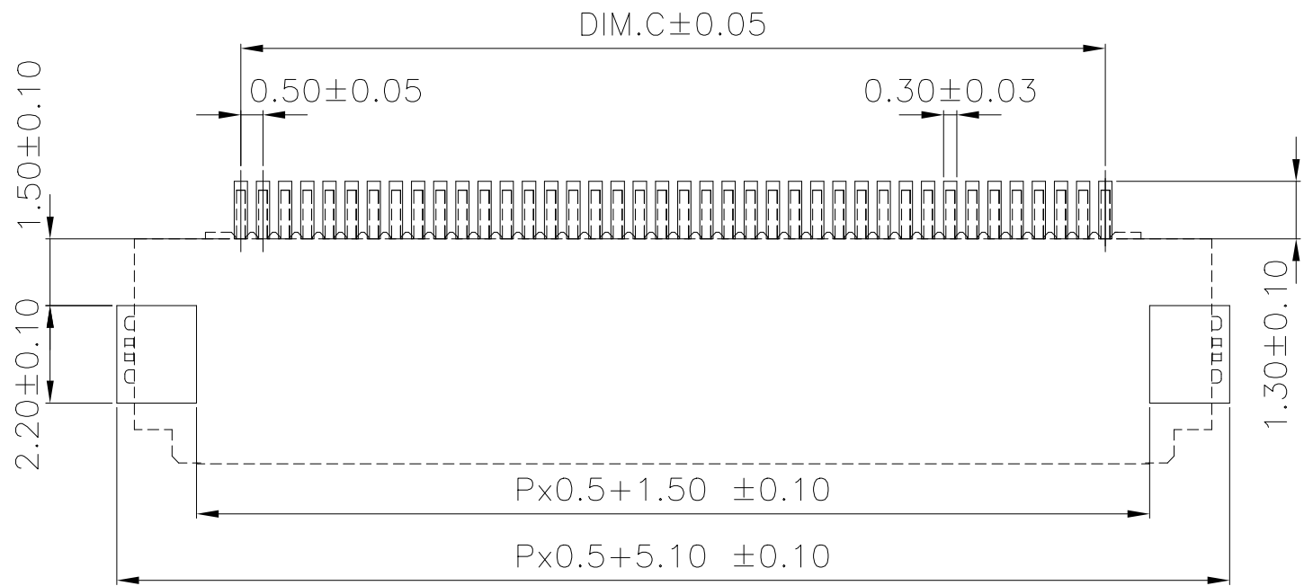
RECOMMENDED P.C. BOARD PATTERN LAYOUT RECOMMENDED METAL MASK THICKNESS: T=0.15
