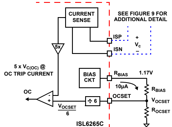
FIGURE 11. OC TRIP CIRCUITRY
