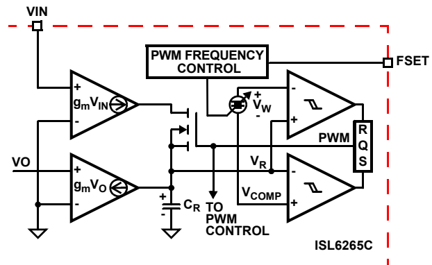
FIGURE 6. MODULATOR CIRCUITRY
