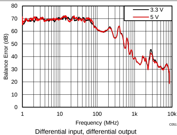
Figure 51. Balance Error
