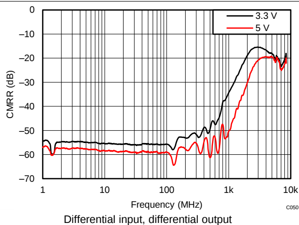
Figure 50. CMRR (Sdc21)
