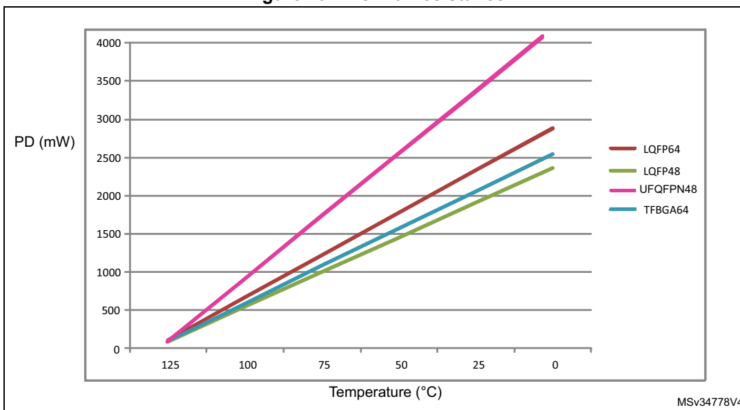
Figure 49. Thermal resistance
