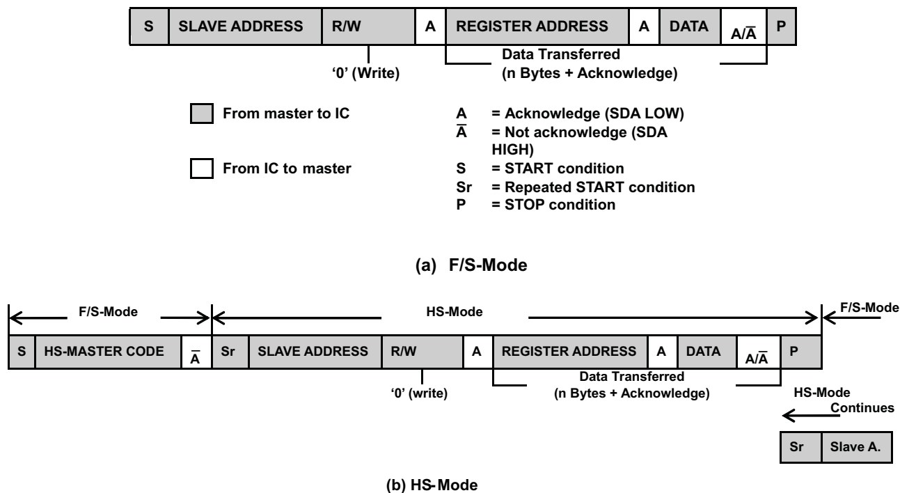
Figure 35. Data Transfer Format in F/S Mode and H/S Mode
