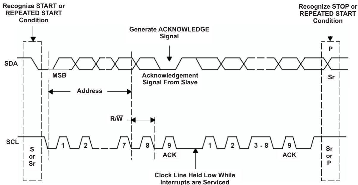
Figure 34. Bus Protocol
