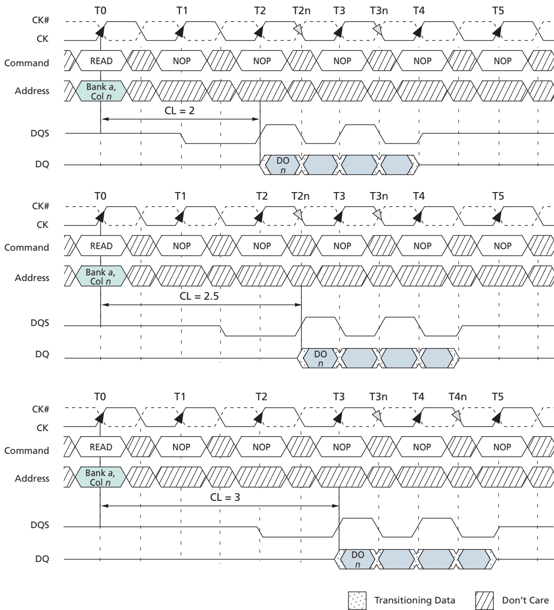
Figure 26: READ Burst
