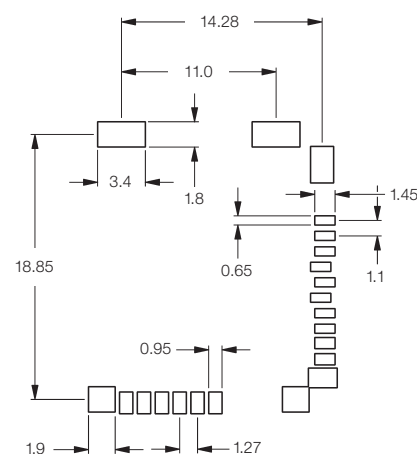
PCB Layout
