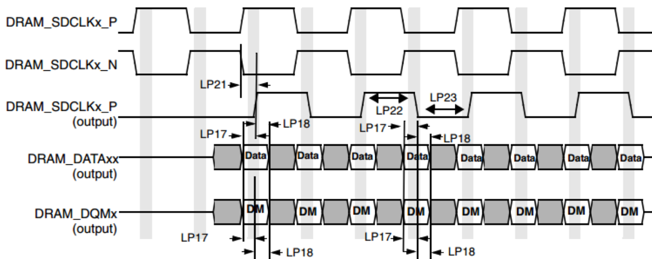
Figure 28. LPDDR3 write cycle
