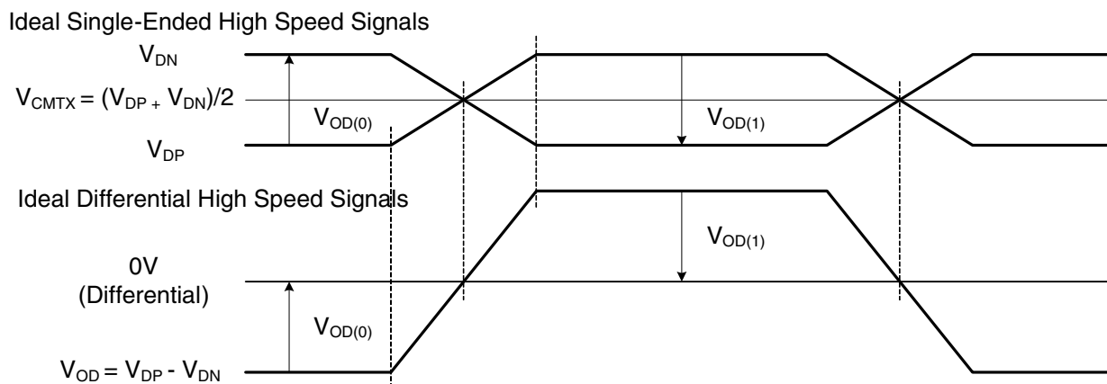
Figure 65. Ideal Single-ended and Resulting Differential HS Signals
