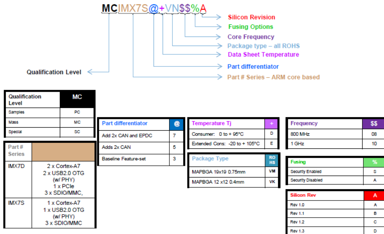
Figure 1. Part number nomenclature—i.MX 7Solo family of processors
