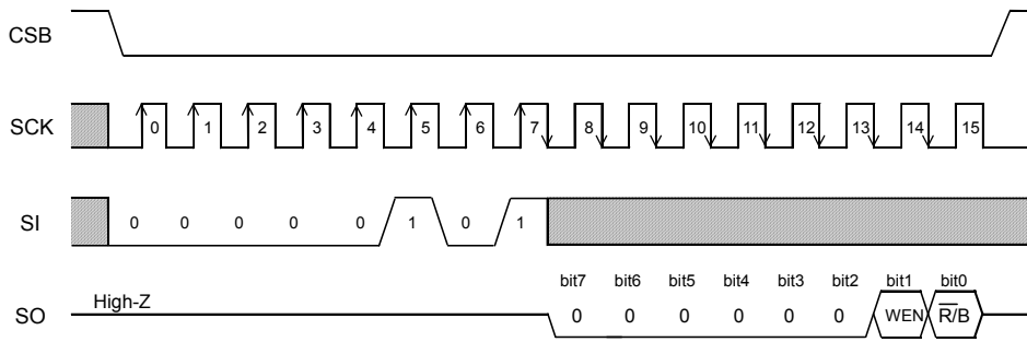
Fig.38 Status register read command (BR35H160/320/640/128-WC)
