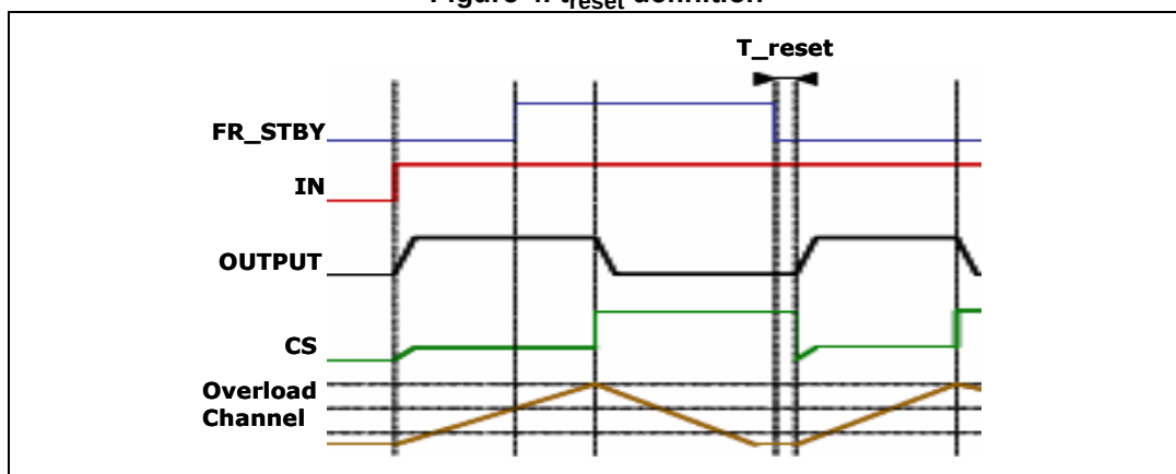
Figure 4. t_{reset} definition
