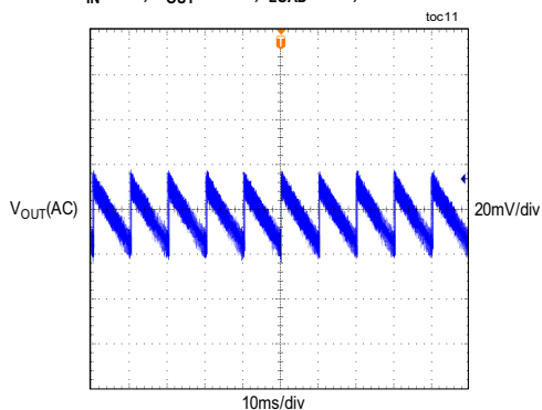
MAXM17624 OUTPUT VOLTAGE RIPPLE V_{IN} = 5V , V_{OUT} = 3.3V , I_{LOAD} = 0A , PFM MODE
