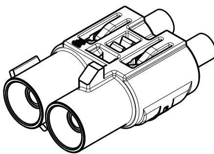
ISOMETRIC VIEW SCALE 2:1
