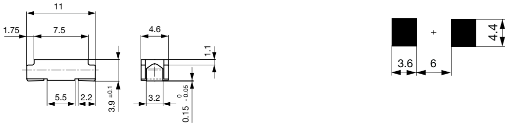
Soldering pads
