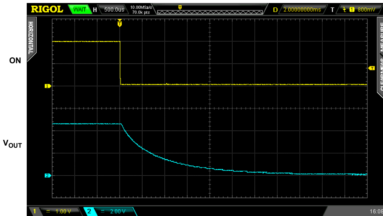
Figure 6. Typical Turn OFF operation waveform for V_{IN} = 4.5\text{ V} , C_{SLEW} = 10\text{ nF} , C_{LOAD} = 10\text{ }\mu\text{F} , R_{LOAD} = 100\text{ }\Omega
