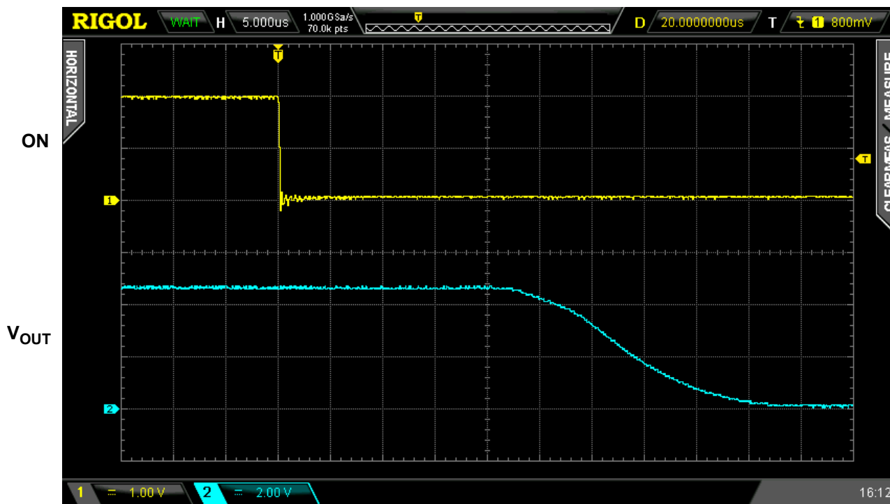
Figure 5. Typical Turn OFF operation waveform for V_{IN} = 4.5\text{ V} , C_{SLEW} = 10\text{ nF} , no C_{LOAD} , R_{LOAD} = 100\text{ }\Omega
