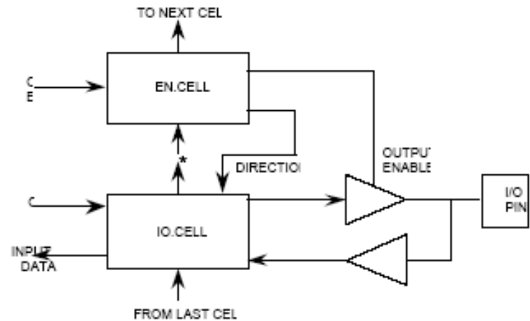
Figure 21-7. General Arrangement for Bidirectional Pins
