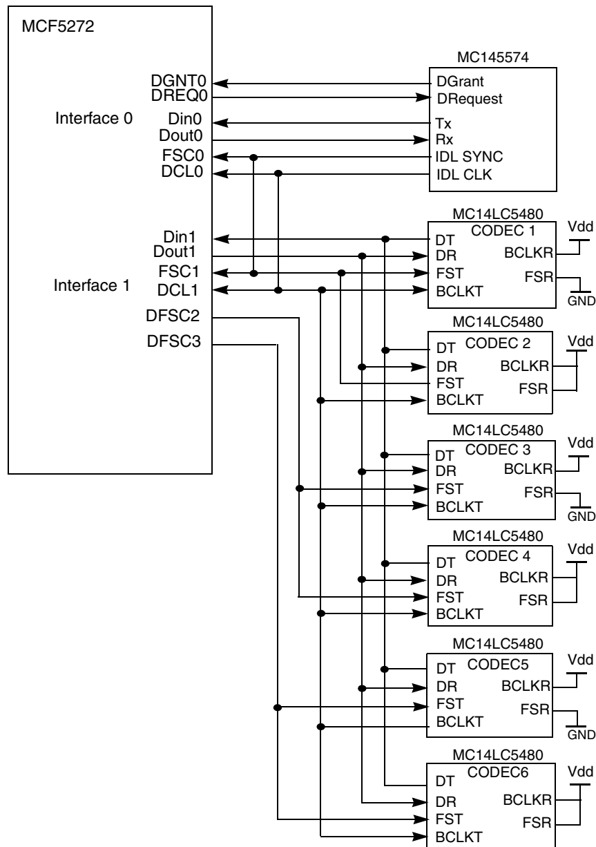
Figure 13-37. ISDN SOHO PABX Example
