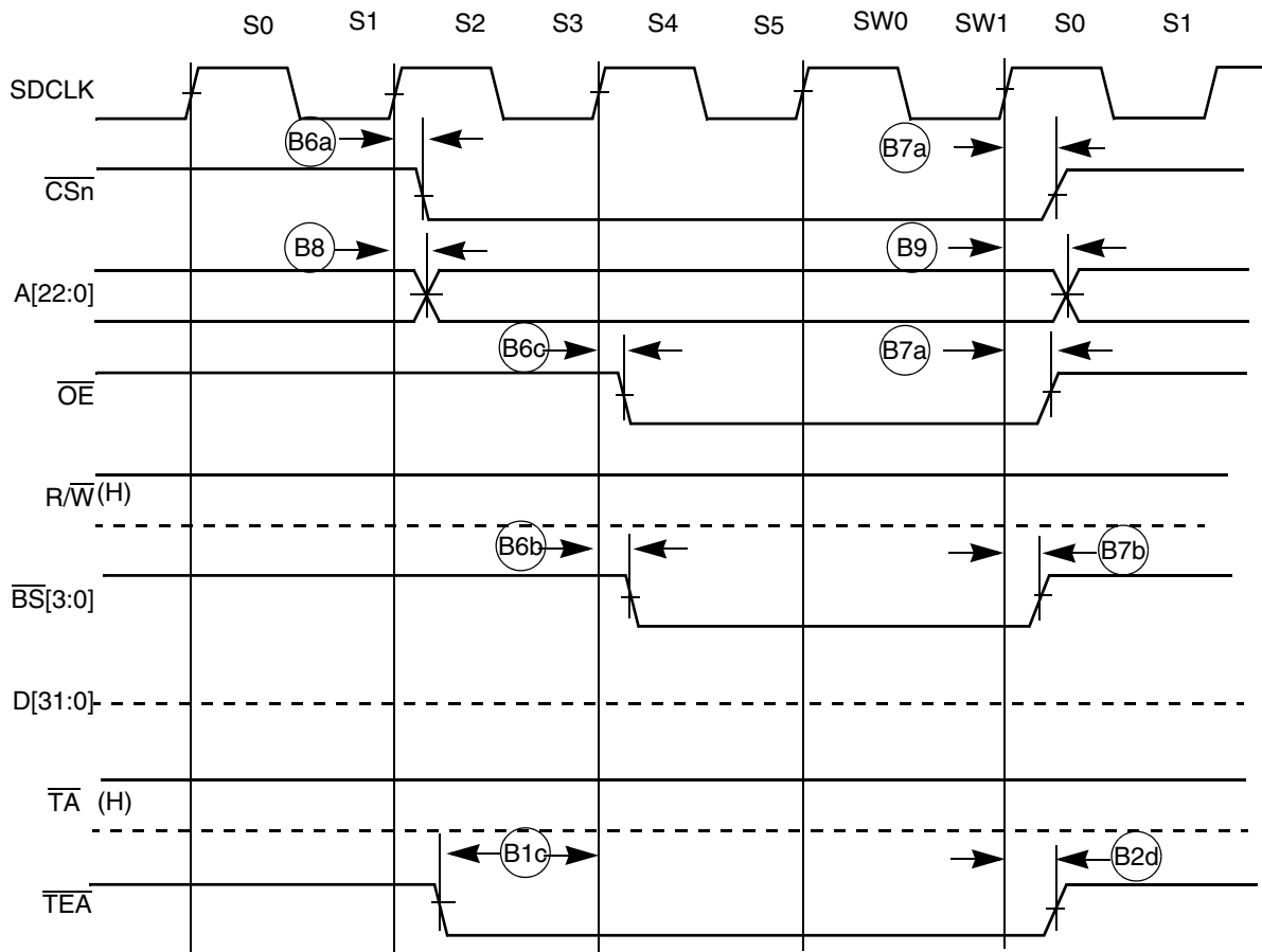
Figure 23-5. SRAM Bus Cycle Terminated by \overline{TEA}
