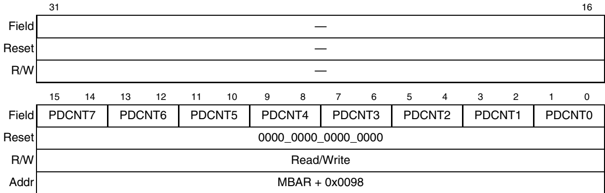
Figure 17-3. Port D Control Register (PDCNT)
