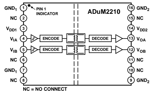
Figure 1. ADuM2210
