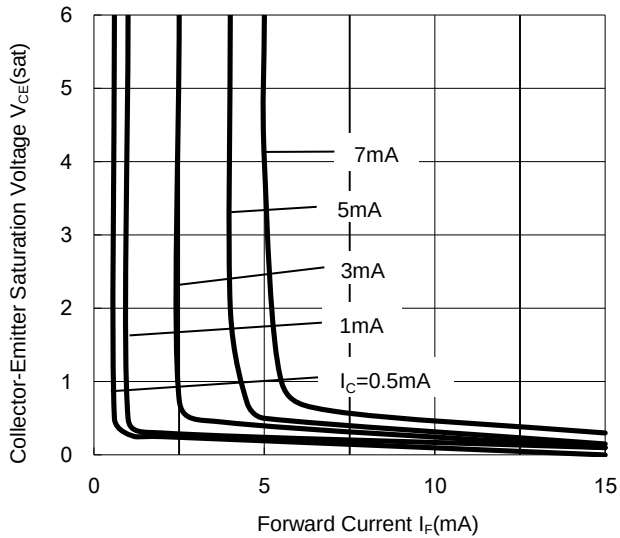
Fig.3 Collector-Emitter Saturation Voltage vs Forward Current
