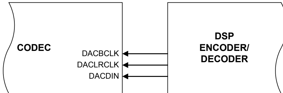
Figure 13. Slave mode
