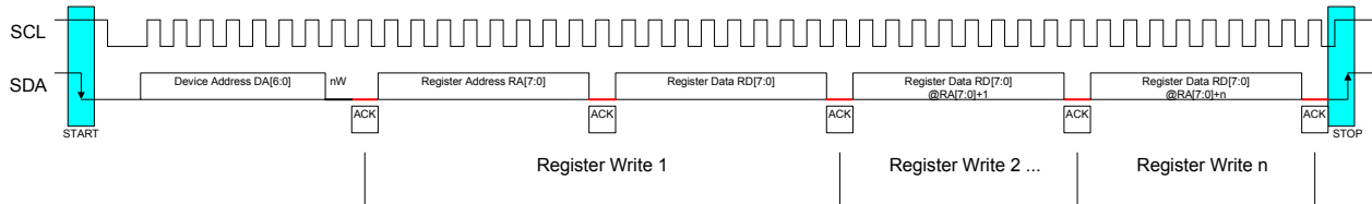
Figure 19. Multiple Write Cycle
