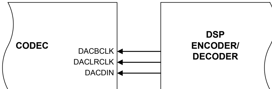
Figure 13. Slave mode
