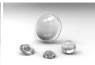
▶ Convex Lens
