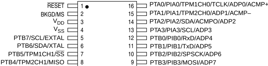
Figure 2-3. 16-Pin TSSOP
