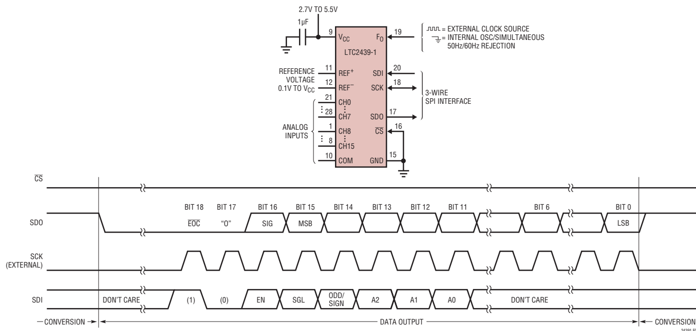
Figure 8. External Serial Clock, \overline{CS} = 0 Operation
