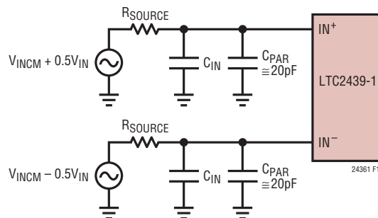
Figure 13. An RC Network at IN^+ and IN^-
