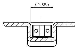
SECT. E-E
