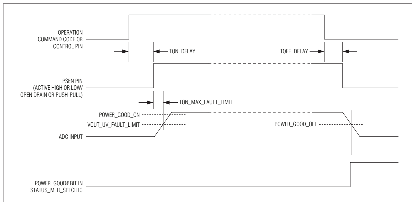
Figure 1. Power-Supply Sequencing
