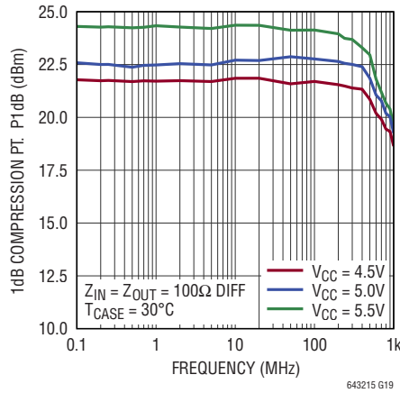
P1dB vs Frequency Over Supply Voltage
