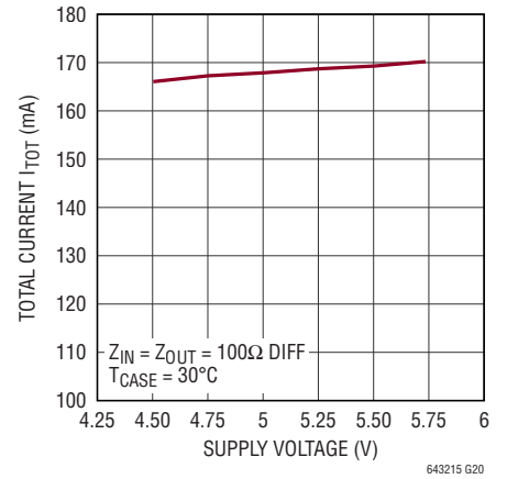
Total Current vs Supply Voltage
