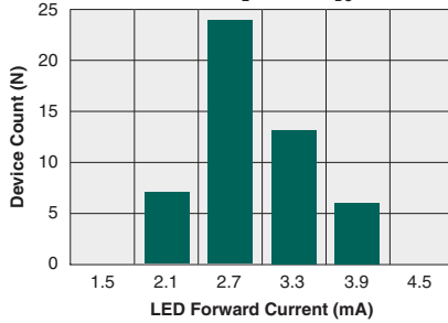
Typical I F for Switch Operation (N=50, I L =250mA DC )
