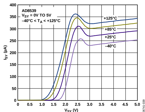
Figure 38. AD8539 Supply Current vs. Supply Voltage
