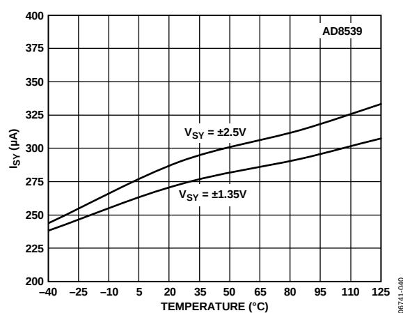
Figure 39. AD8539 Supply Current vs. Temperature
