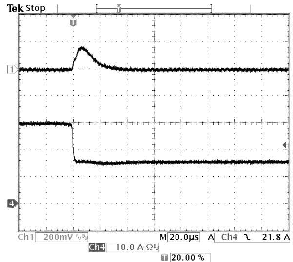
Fig-1.8V-7: Output voltage response for V_{out}=1.8V to negative load current step change from 30A to 15A with slew rate of -5A/us at V_{in}=12V . C_o=47uFx2 ceramic. Top trace: output voltage (200mV/div.) Bottom trace: load current (10A/div.) Time scale: 20us/div.
