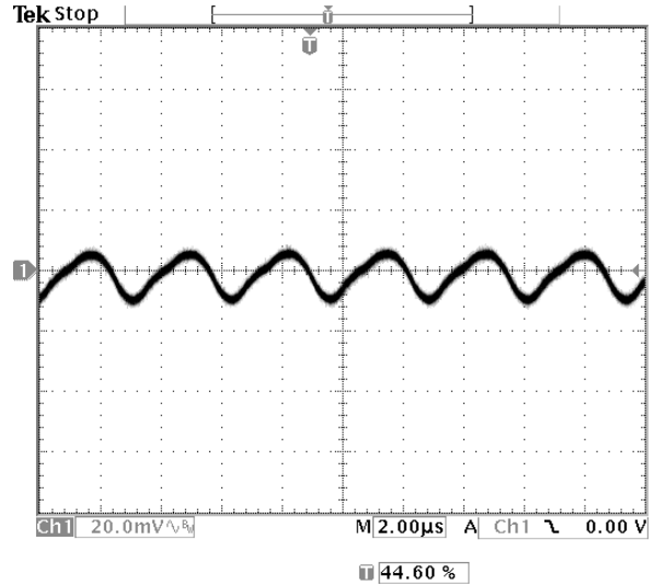
Fig-3.3V-5: Output voltage ripple (20mV/div.) for V_{out}=3.3V at full rated load current into a resistive load with external capacitance 47\mu F \times 2 ceramic + 1\mu F ceramic at V_{in}=12V . Time scale: 2 us/div
