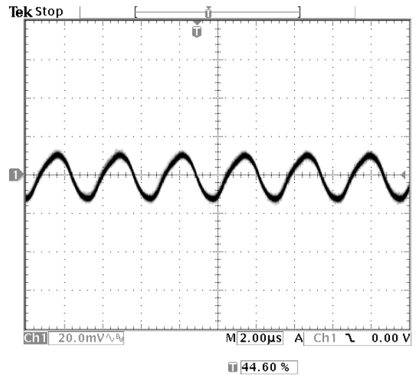
Fig-5.0V-5: Output voltage ripple (20mV/div.) for Vout=5.0V at full rated load current into a resistive load with external capacitance 47uFx2 ceramic + 1uF ceramic at Vin=12V. Time scale: 2 us/div
