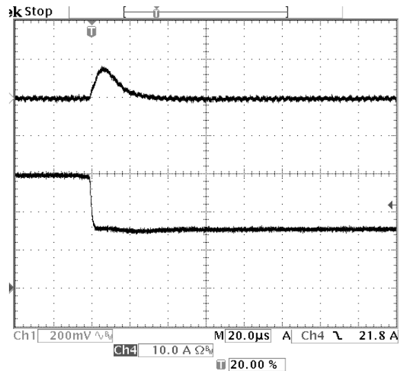
Fig-2.0V-7: Output voltage response for V_{out}=2.0V to negative load current step change from 30A to 15A with slew rate of -5A/\mu s at V_{in}=12V . C_o=47\mu F \times 2 ceramic. Top trace: output voltage (200mV/div.) Bottom trace: load current (10A/div.) Time scale: 20us/div.
