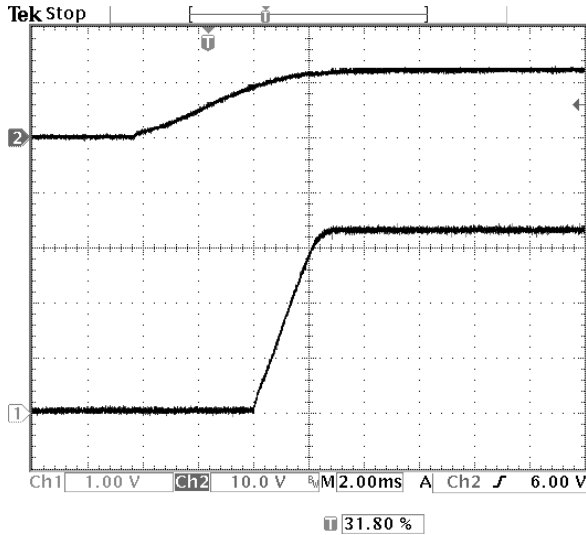
Fig-3.3V-4: Turn-on transient for V_{out}=3.3V with application of V_{in} at full rated load current (resistive) and 47\mu F \times 2 external capacitance at V_{in}=12V . Top trace: V_{in} (10V/div.) Bottom trace: output voltage (1V/div.) Time scale: 2ms/div.
