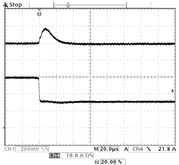
Fig-1.5V-7: Output voltage response for Vout=1.5V to negative load current step change from 30A to 15A with slew rate of -5A/us at Vin=12V. Co=47uFx2 ceramic. Top trace: output voltage (200mV/div.) Bottom trace: load current (10A/div.) Time scale: 20us/div.
