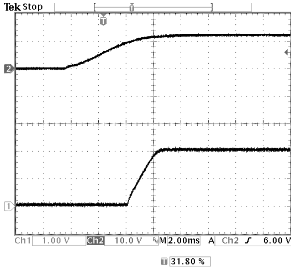
Fig-2.0V-4: Turn-on transient for V_{out}=2.0V with application of V_{in} at full rated load current (resistive) and 47\mu F \times 2 external capacitance at V_{in}=12V . Top trace: V_{in} (10V/div.) Bottom trace: output voltage (1V/div.) Time scale: 2 ms/div.
