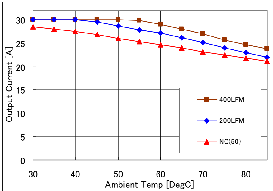
Fig-1.8V-1: Available load current vs. ambient temperature and airflow rates for Vout=1.8V with Vin=12V. Maximum component temperature ≤ 120°C
