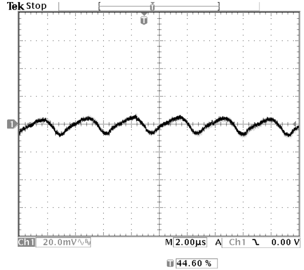
Fig-2.5V-5: Output voltage ripple (20mV/div.) for V_{out}=2.5V at full rated load current into a resistive load with external capacitance 47\mu F \times 2 ceramic + 1uF ceramic at V_{in}=12V . Time scale: 2 us/div
