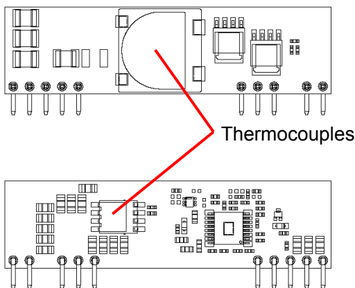
Fig. D: Location of the thermo couples for thermal testing
