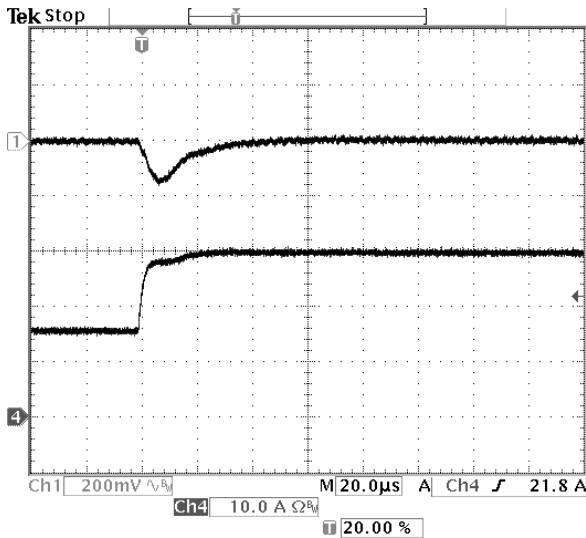
Fig-1.5V-6: Output voltage response for Vout=1.5V to positive load current step change from 15A to 30A with slew rate of 5A/us at Vin=12V. Co=47uFx2 ceramic. Top trace: output voltage (200mV/div.) Bottom trace: load current (10A/div.) Time scale: 20us/div.
