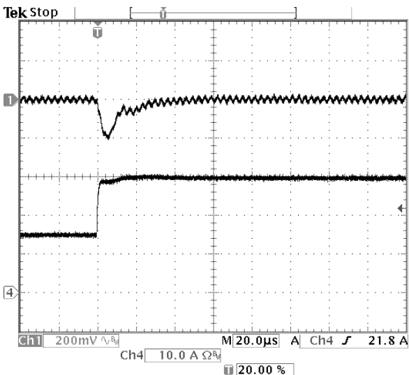
Fig-5.0V-6: Output voltage response for Vout=5.0V to positive load current step change from 15A to 30A with slew rate of 5A/us at Vin=12V. Co=47uFx2 ceramic. Top trace: output voltage (200mV/div.) Bottom trace: load current (10A/div.) Time scale: 20us/div.
