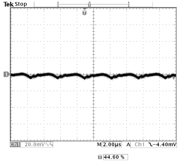
Fig-1.0V-5: Output voltage ripple (20mV/div.) for V_{out}=1.0V at full rated load current into a resistive load with external capacitance 47\mu F \times 2 ceramic + 1\mu F ceramic at V_{in}=12V . Time scale: 2 us/div
