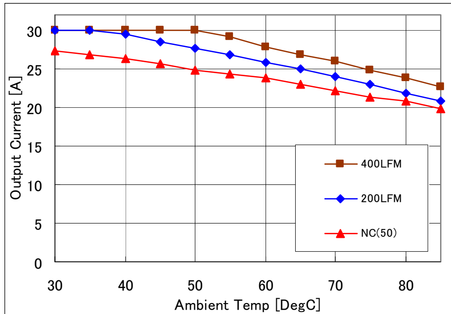
Fig-3.3V-1: Available load current vs. ambient temperature and airflow rates for Vout=3.3V with Vin=12V. Maximum component temperature ≤ 120°C.
