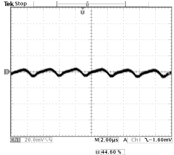
Fig-2.0V-5: Output voltage ripple (20mV/div.) for V_{out}=2.0V at full rated load current into a resistive load with external capacitance 47\mu F \times 2 ceramic + 1\mu F ceramic at V_{in}=12V . Time scale: 2 us/div
