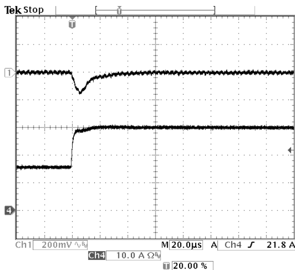
Fig-2.5V-6: Output voltage response for V_{out}=2.5V to positive load current step change from 15A to 30A with slew rate of 5A/us at V_{in}=12V . C_o=47\mu F \times 2 ceramic. Top trace: output voltage (200mV/div.) Bottom trace: load current (10A/div.) Time scale: 20us/div.
