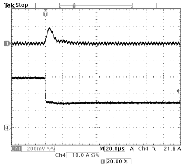
Fig-5.0V-7: Output voltage response for Vout=5.0V to negative load current step change from 30A to 15A with slew rate of -5A/us at Vin=12V. Co=47uFx2 ceramic. Top trace: output voltage (200mV/div.) Bottom trace: load current (10A/div.) Time scale: 20us/div.
