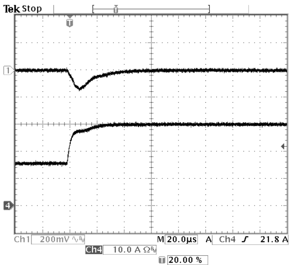
Fig-1.0V-6: Output voltage response for V_{out}=1.0V to positive load current step change from 15A to 30A with slew rate of 5A/\mu s at V_{in}=12V . C_o=47\mu F \times 2 ceramic. Top trace: output voltage (200mV/div.) Bottom trace: load current (10A/div.) Time scale: 20us/div.
