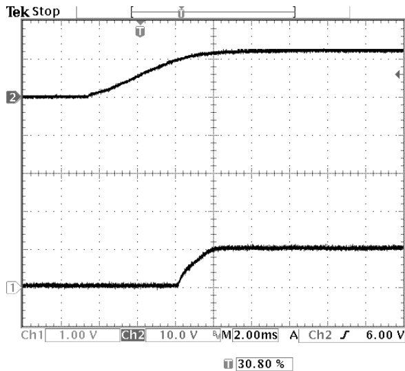
Fig-1.0V-4: Turn-on transient for V_{out}=1.0V with application of V_{in} at full rated load current (resistive) and 47\mu F \times 2 external capacitance at V_{in}=12V . Top trace: V_{in} (10V/div.) Bottom trace: output voltage (1V/div.) Time scale: 2 ms/div.
