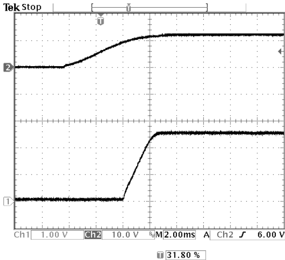
Fig-2.5V-4: Turn-on transient for V_{out}=2.5V with application of V_{in} at full rated load current (resistive) and 47\mu F \times 2 external capacitance at V_{in}=12V . Top trace: V_{in} (10V/div.) Bottom trace: output voltage (1V/div.) Time scale: 2 ms/div.
