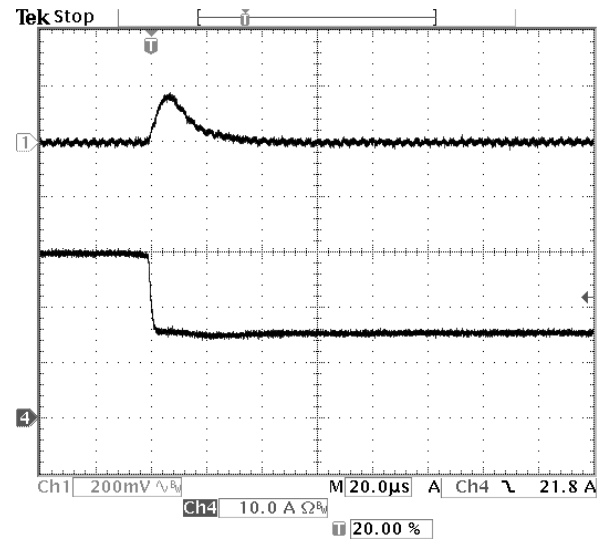
Fig-2.5V-7: Output voltage response for V_{out}=2.5V to negative load current step change from 30A to 15A with slew rate of -5A/us at V_{in}=12V . C_o=47\mu F \times 2 ceramic. Top trace: output voltage (200mV/div.) Bottom trace: load current (10A/div.) Time scale: 20us/div.
