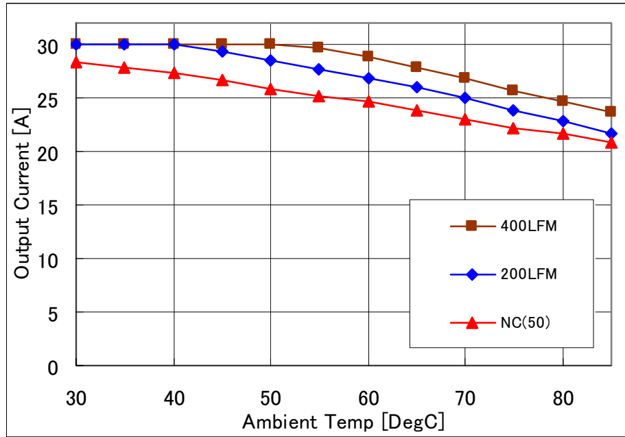
Fig-2.0V-1: Available load current vs. ambient temperature and airflow rates for Vout=2.0V with Vin=12V. Maximum component temperature \leq 120^{\circ}\text{C}
