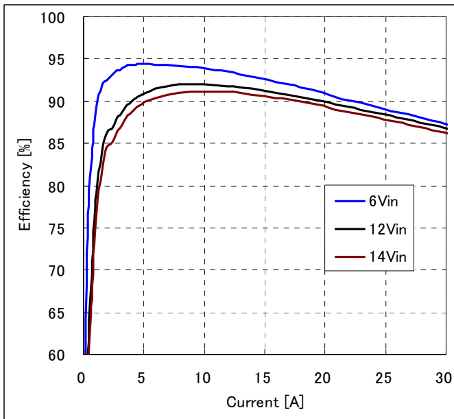
Fig-1.8V-2: Efficiency vs. load current and input voltage for Vout=1.8V. Airflow rate=200 LFM (1m/s) and Ta=25°C.
