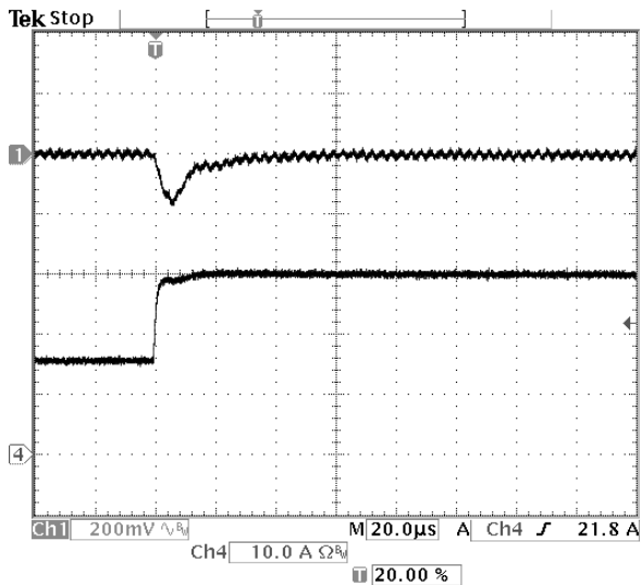
Fig-3.3V-6: Output voltage response for V_{out}=3.3V to positive load current step-change from 15A to 30A with slew rate of 5A/\mu s at V_{in}=12V . C_o=47\mu F \times 2 ceramic. Top trace: output voltage (200mV/div.) Bottom trace: load current (10A/div.) Time scale: 20us/div.
