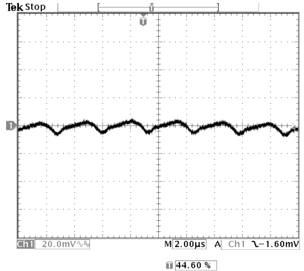
Fig-1.8V-5: Output voltage ripple (20mV/div.) for V_{out}=1.8V at full rated load current into a resistive load with external capacitance 47uFx2 ceramic + 1uF ceramic at V_{in}=12V . Time scale: 2 us/div
