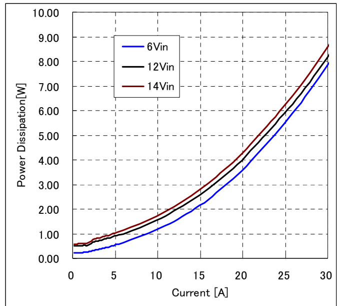
Fig-1.8V-3: Power Loss vs. load current and input voltage for Vout=1.8V. Airflow rate=200 LFM (1.0 m/s) and Ta=25°C.
