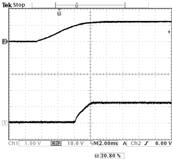
Fig-1.2V-4: Turn-on transient for V_{out}=1.2V with application of V_{in} at full rated load current (resistive) and 47uFx2 external capacitance at V_{in}=12V . Top trace: V_{in} (10V/div.) Bottom trace: output voltage (1V/div.) Time scale: 2ms/div.
