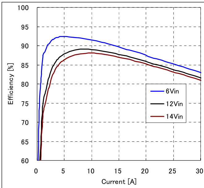
Fig-1.2V-2: Efficiency vs. load current and input voltage for Vout=1.2V. Airflow rate=200 LFM (1m/s) and Ta=25°C.
