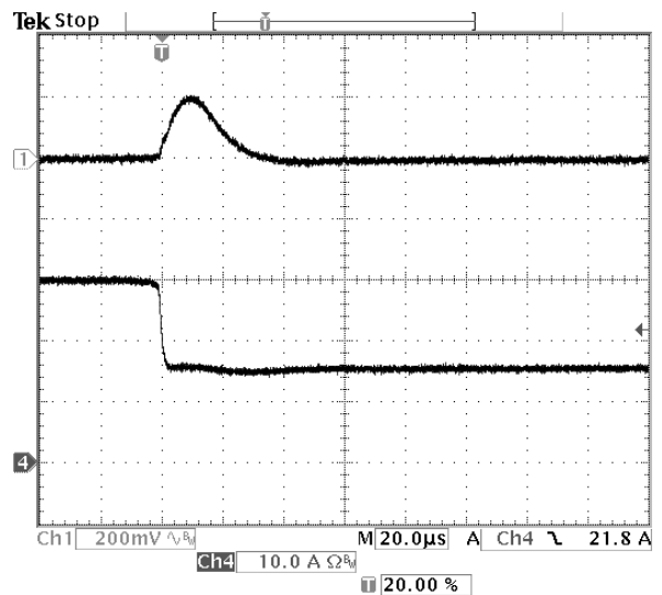
Fig-1.0V-7: Output voltage response for V_{out}=1.0V to negative load current step change from 30A to 15A with slew rate of -5A/\mu s at V_{in}=12V . C_o=47\mu F \times 2 ceramic. Top trace: output voltage (200mV/div.) Bottom trace: load current (10A/div.) Time scale: 20us/div.
