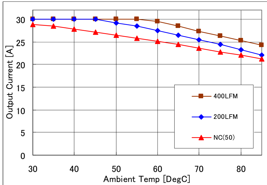
Fig-1.2V-1: Available load current vs. ambient temperature and airflow rates for Vout=1.2V with Vin=12V. Maximum component temperature ≤ 120°C
