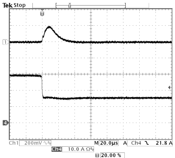
Fig-1.2V-7: Output voltage response for V_{out}=1.2V to negative load current step change from 30A to 15A with slew rate of -5A/us at V_{in}=12V . C_o=47uFx2 ceramic. Top trace: output voltage (200mV/div.) Bottom trace: load current (10A/div.) Time scale: 20us/div.
