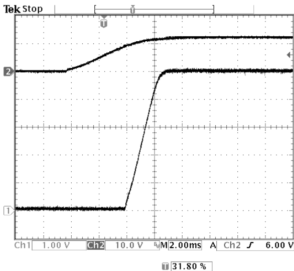
Fig-5.0V-4: Turn-on transient for Vout=5.0V with application of Vin at full rated load current (resistive) and 47uFx2 external capacitance at Vin=12V. Top trace: Vin (10V/div.) Bottom trace: output voltage (1V/div.) Time scale: 2 ms/div.
