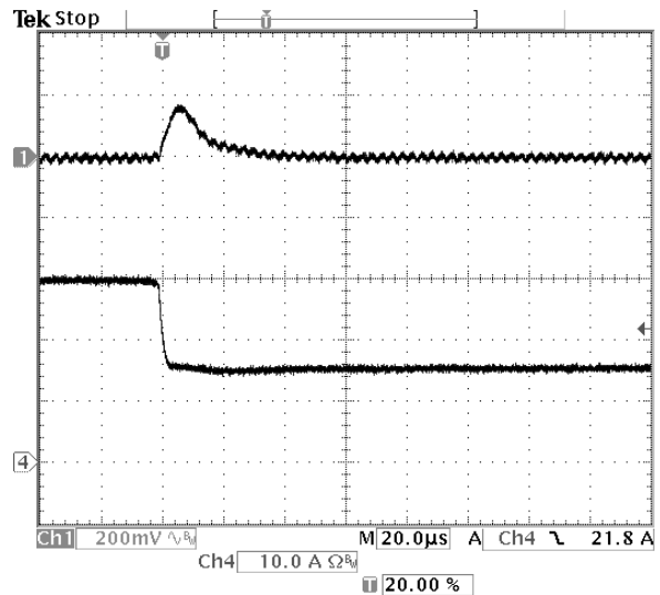
Fig-3.3V-7: Output voltage response for V_{out}=3.3V to negative load current step change from 30A to 15A with slew rate of -5A/\mu s at V_{in}=12V . C_o=47\mu F \times 2 ceramic. Top trace: output voltage (200mV/div.) Bottom trace: load current (10A/div.) Time scale: 20us/div.
