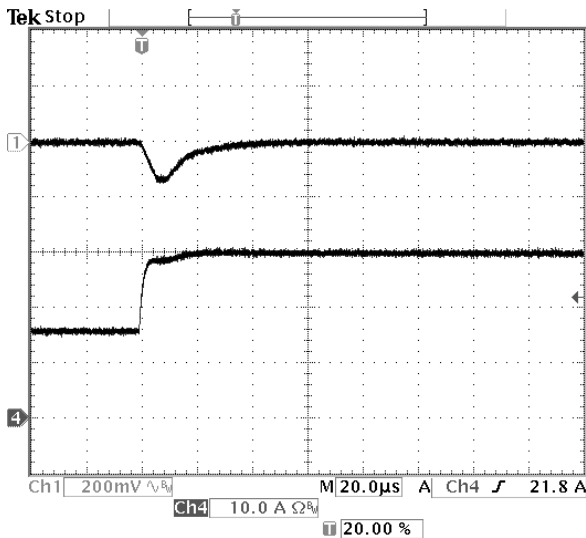
Fig-2.0V-6: Output voltage response for V_{out}=2.0V to positive load current step change from 15A to 30A with slew rate of 5A/\mu s at V_{in}=12V . C_o=47\mu F \times 2 ceramic. Top trace: output voltage (200mV/div.) Bottom trace: load current (10A/div.) Time scale: 20us/div.
