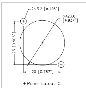
C TYPE PANEL CUTOUT
