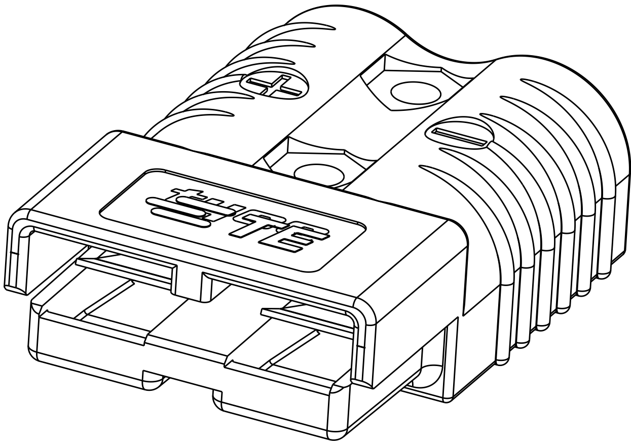
PART NUMBER: 1604043-2 WITHOUT CONTACT SHOWN
