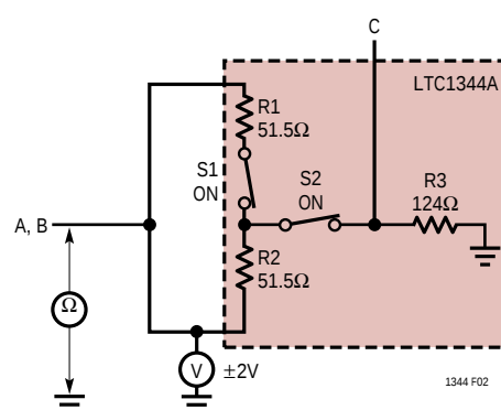
Figure 2. V.35 Common Mode Impedance Measurement
