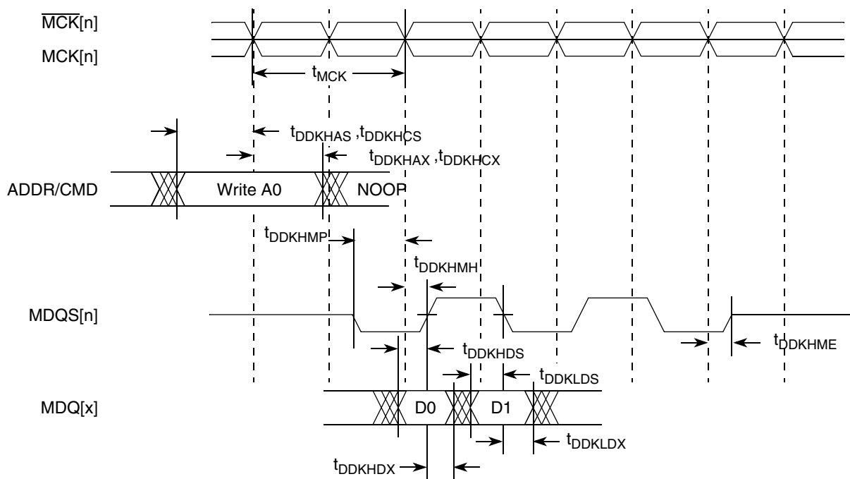
Figure 6 shows the DDR SDRAM output timing diagram.
