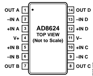
Figure 3. 14-Lead TSSOP
