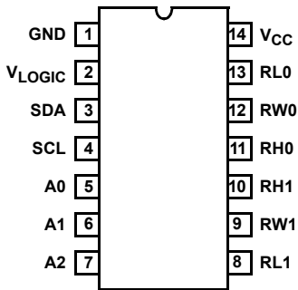
ISL23325 (14 LD TSSOP) TOP VIEW
