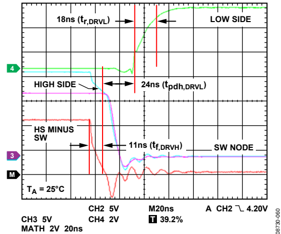
Figure 61. Upper-Side Driver Falling and Lower-Side Rising Edge Waveforms ( C_{IN} = 4.3 nF (Upper-/Lower-Side MOSFET), Q_{TOTAL} = 27 nC ( V_{GS} = 4.4 V (Q1), V_{GS} = 5 V (Q3))
