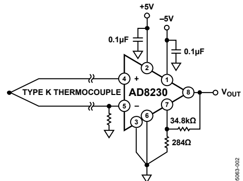
Figure 3. Thermocouple Measurement
