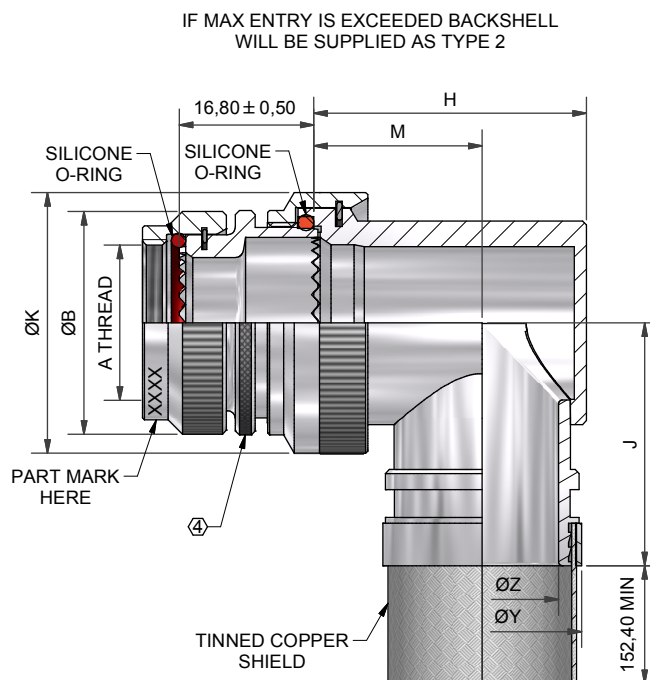
90° BACKSHELL - TYPE 2
