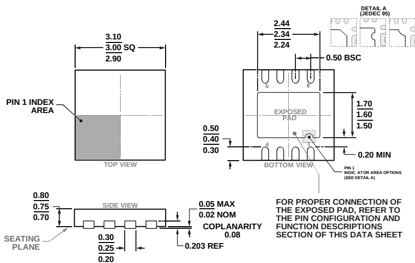
Figure 80. 8-Lead Lead Frame Chip Scale Package [LFCSP] 3 mm x 3 mm Body and 0.75 mm Package Height (CP-8-11)
