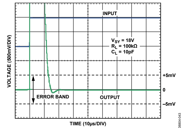
Figure 55. Positive Settling Time to 0.1%
