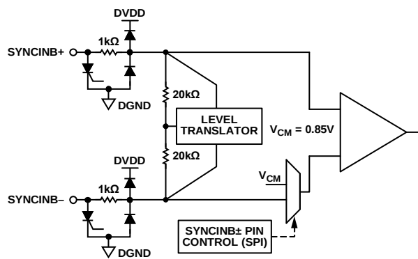
Figure 108. SYNCINB± Inputs
