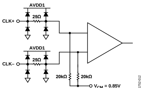
Figure 105. Clock Inputs
