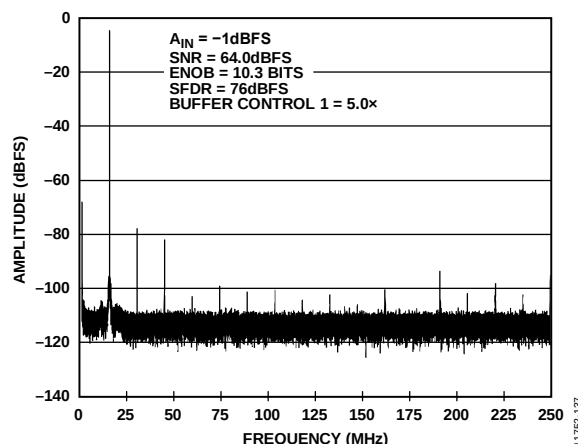
Figure 85. Single-Tone FFT with f_{IN} = 985.3 MHz
