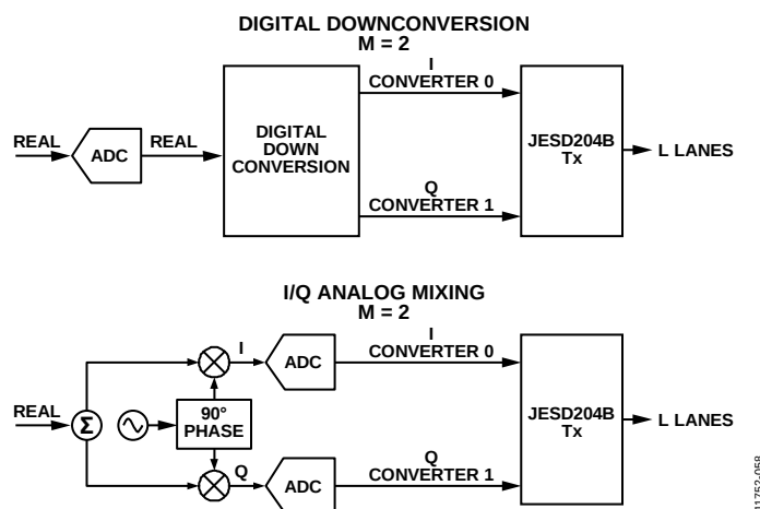
Figure 167. I/Q Transport Layer Mapping
