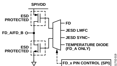
Figure 112. FD_A/FD_B Outputs
