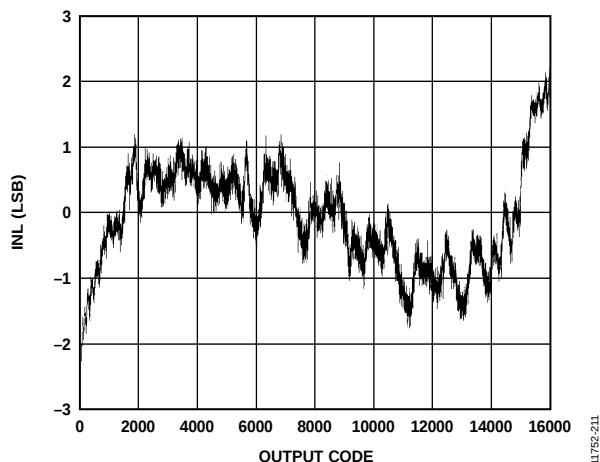
Figure 50. INL, f_{IN} = 10.3 MHz
