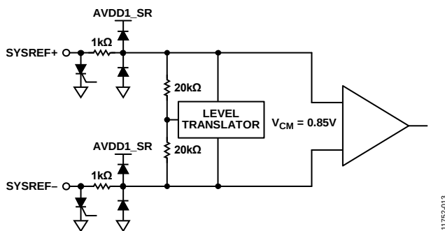
Figure 106. SYSREF± Inputs
