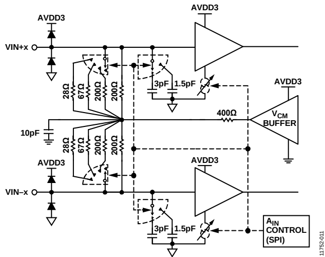
Figure 104. Analog Inputs
