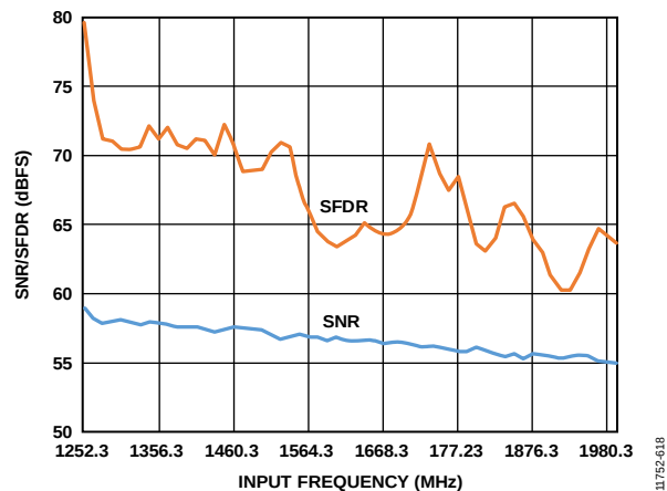
Figure 18. SNR/SFDR vs. f_{IN} ; 1.3 \text{ GHz} < f_{IN} < 2 \text{ GHz} ; Buffer Control 1 (0x018) = 8.5×
