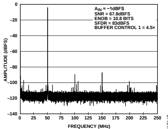
Figure 83. Single-Tone FFT with f_{IN} = 450.3 MHz
