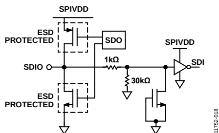
Figure 111. SDIO Input
