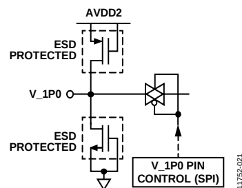
Figure 114. V_1P0 Input/Output
