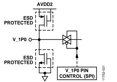
Figure 114. V_1P0 Input/Output
