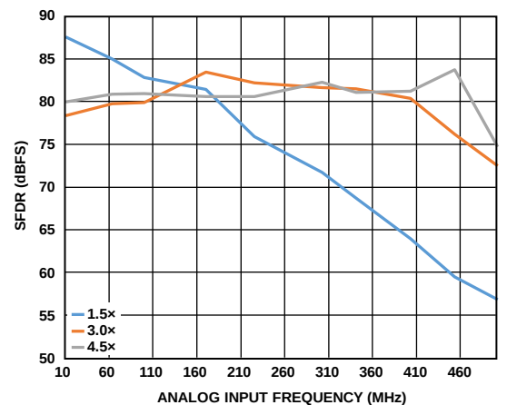
Figure 121. Buffer Current Sweeps, AD9680-1000 (SFDR vs. I_{BUFF} ); f_{IN} < 500 MHz; Front-End Network Shown in Figure 115
