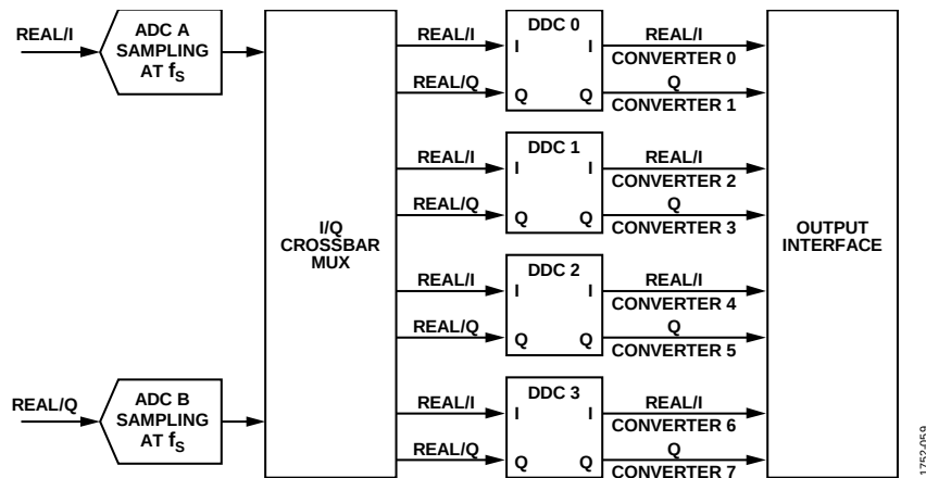
Figure 168. DDCs and Virtual Converter Mapping
