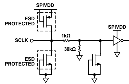
Figure 109. SCLK Input
