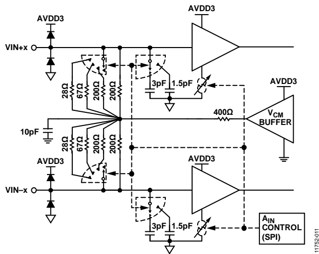
Figure 104. Analog Inputs
