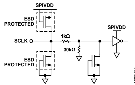
Figure 109. SCLK Input
